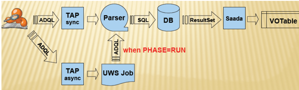
Figure 5: The workflow executed by the SSC XMM Obs/Tap service for resolving a query. It has two execution modes as required for TAP: a synchronous one , top branch and an asynchronous one, using the UWS protocol.
