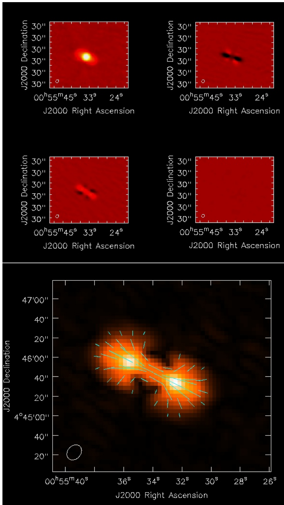
Figure 2: VLA images of Jupiter at 1.4 GHz. From left to right: Top row, Stokes I (total intensity), Stokes Q. Middle row, Stokes U, V (no signal in V). Bottom, Polarized intensity, with polarization vectors overlaid.
