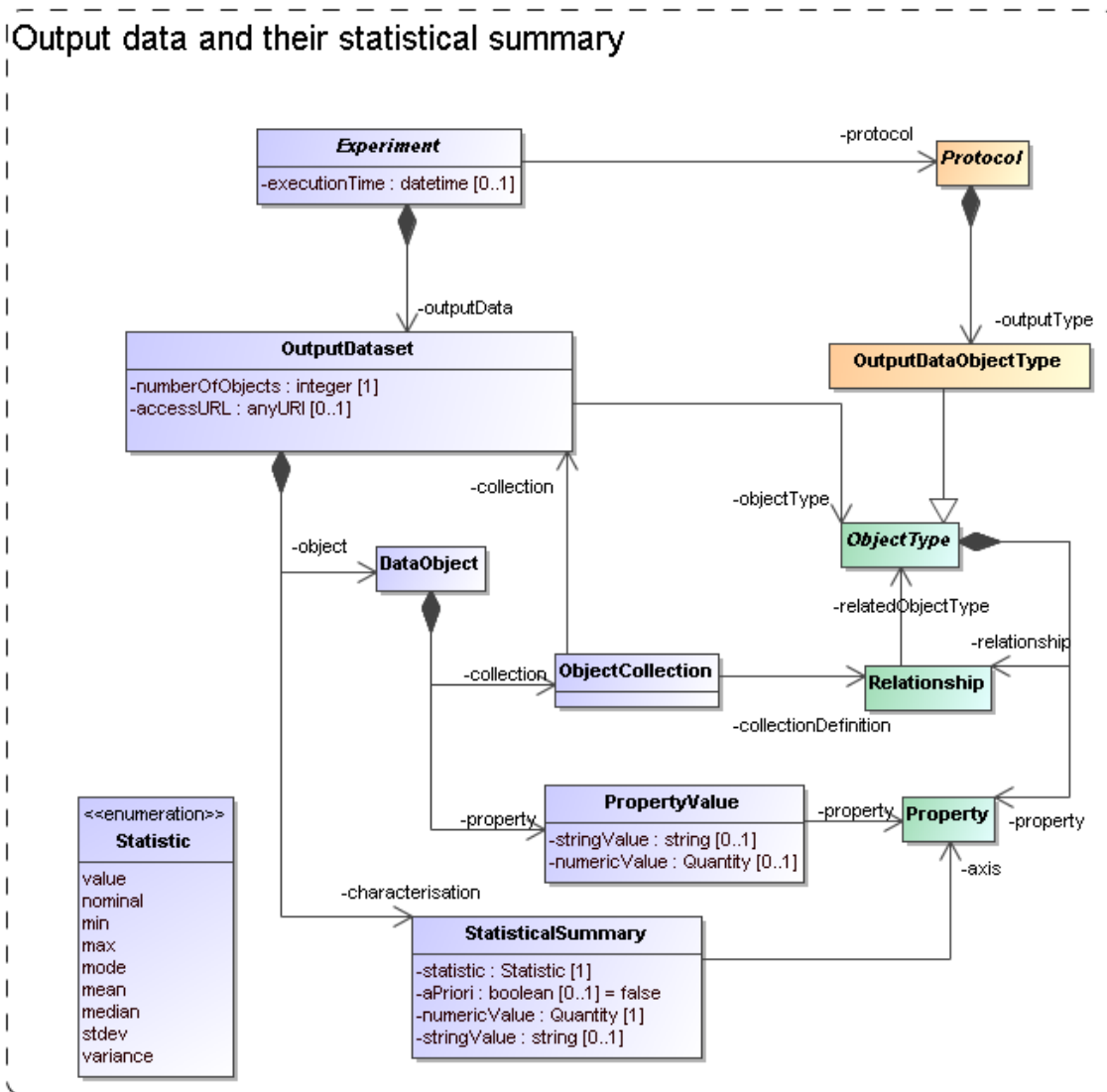
Figure 11: Modelling Output data sets and their contents.
