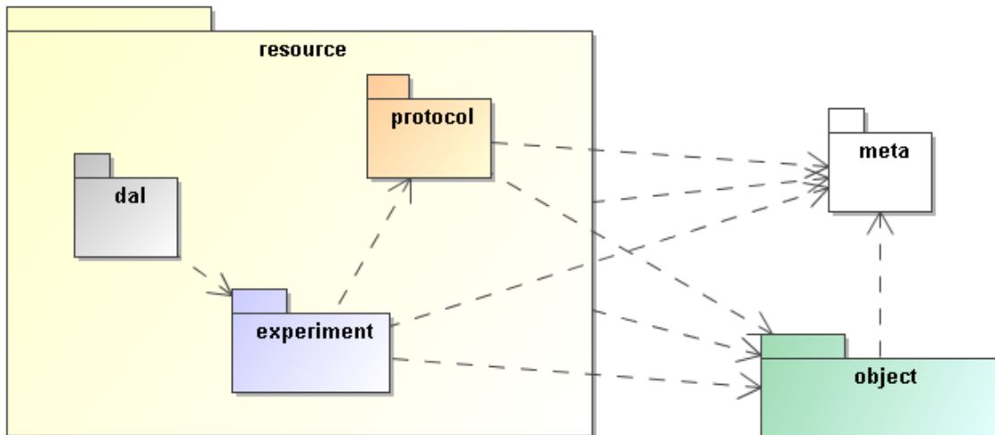
Figure 2: The packages of the SimDM and their relationships. These are related to each other through directed dependency links indicated by the dashed arrows.
