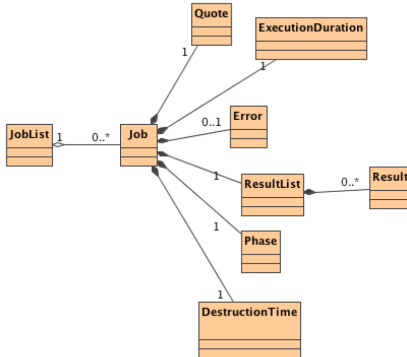
Illustration 1: UWS Objects
